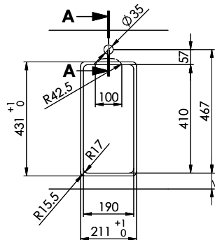
X (1:2)
