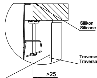
Z (1:1)
