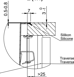
Z (1:1)
